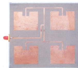
VII. 2x2 Rectangle Microstrip Patch Antenna Array
