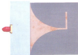
VI. Printed Dipole Antenna Top View Bottom View
