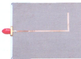
VI. Printed Dipole Antenna Top View Bottom View
