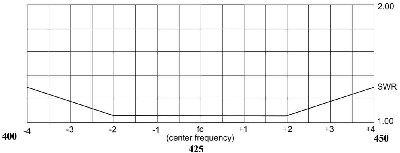
Typical Frequency to SWR Chart
