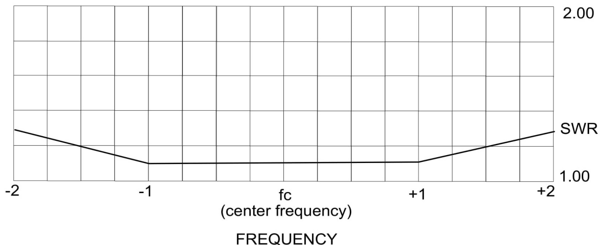
TYPICAL FREQUENCY TO SWR CHART
