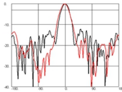
Frequency: 5.0GHz
