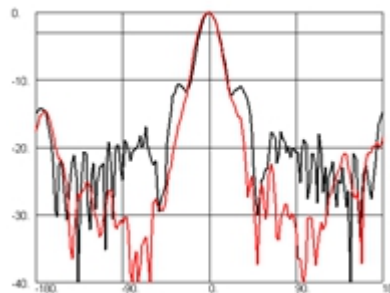
Frequency: 7.0GHz
