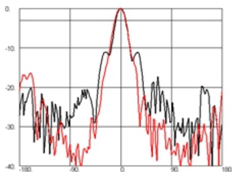
Frequency: 8.0GHz
